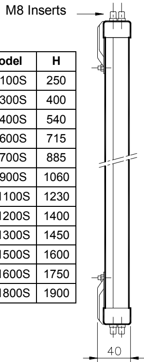
Figure 32 - Fastening brackets for mirrors
